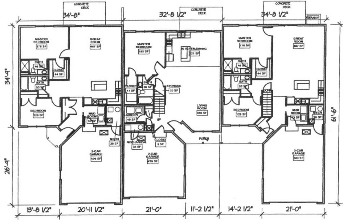
First Floor Plan Building 102
