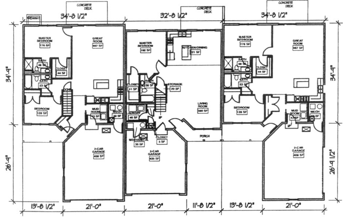
First Floor Plan Buildings 110, 101, 108
